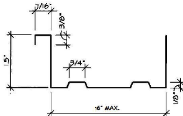
Standing Seam Panel Dimensions
